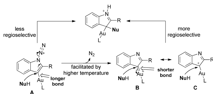
Scheme 2. Rationale for the inverse relationship between regioselectivities and reaction temperatures.
